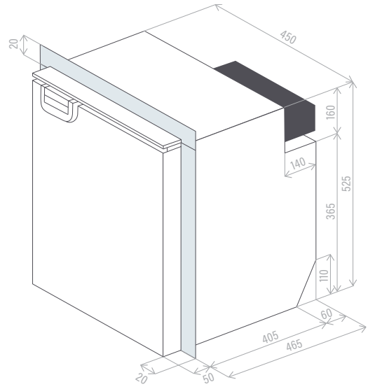
Model DC65-X
