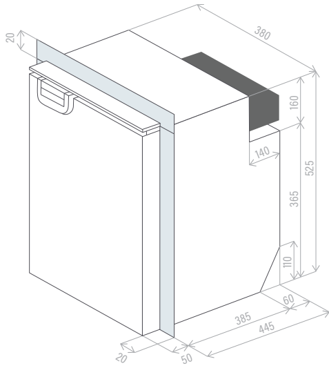
Model DC50-X
