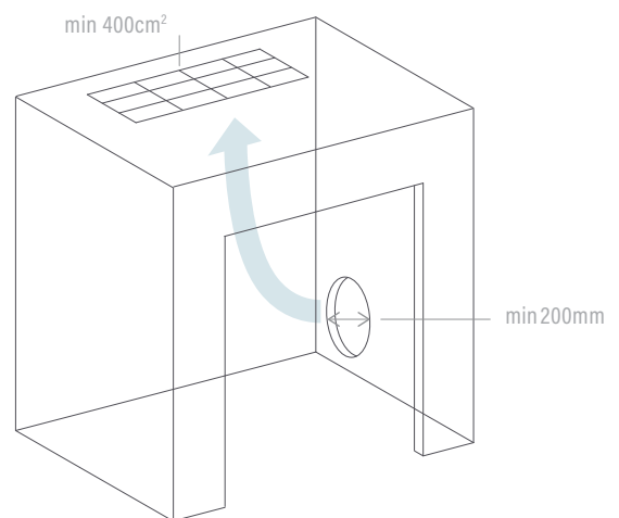
Interior ventilation option 4
