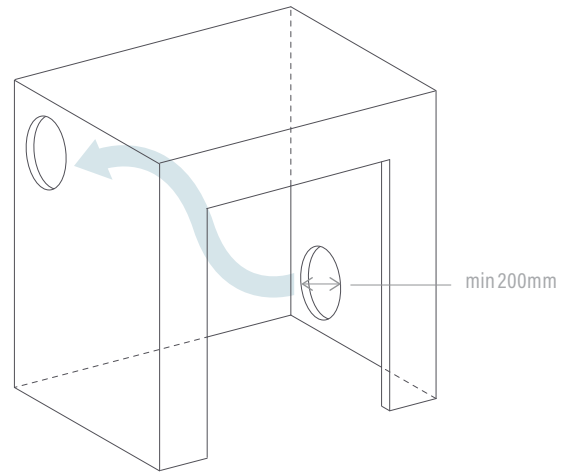
Interior ventilation option 2
