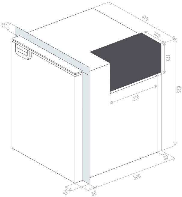
Model DC85-X
