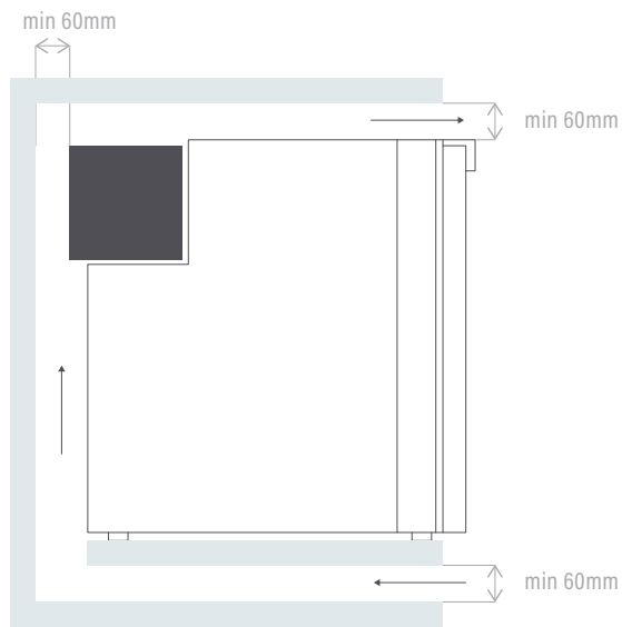
Interior ventilation option 1
