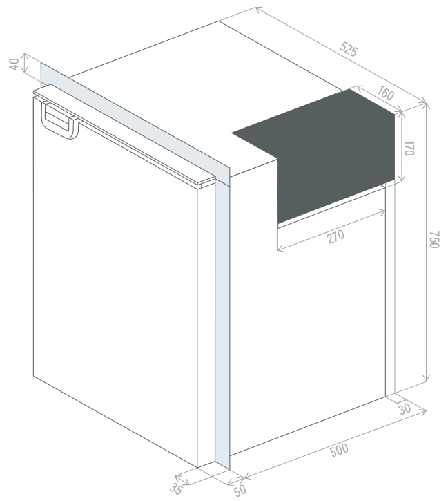
Model DC130-X
